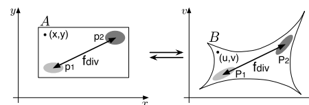
図1 空間写像とそれに不変な f -divergence Fig.1 Feature transformation and transform-invariant f -divergence.
