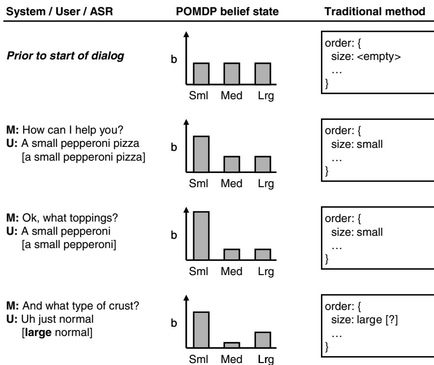
Fig. 12. Example conversation with a spoken dialog system illustrating the benefit of maintaining multiple dialog state hypotheses. This example is in the pizza ordering domain. The left column shows the machine and user utterances, and the recognition results from the user's utterance is shown in brackets. The centre column shows a portion of the POMDP belief state; b represents the belief over a component of the user's goal (pizza size). The right-hand column shows a typical frame-based method which is also tracking this component of the user's goal. Note that a speech recognition error is made in the last turn – this causes the traditional method to absorb a piece of bad information, whereas the POMDP belief state is more robust. In this example no account is taken of which user actions are more or less likely, or of confidence score – see below for illustrations of these elements.
